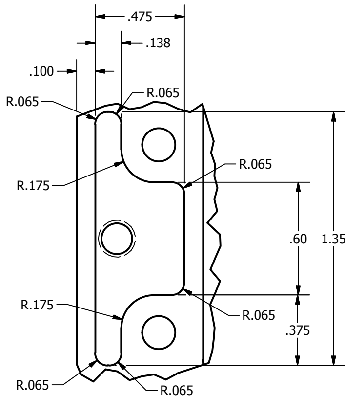
DETAIL C
