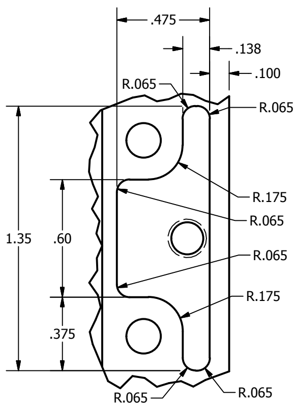
DETAIL D
